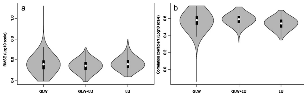
Fig. 3. Violin plots of (a) root mean square error (RMSE) and (b) correlation coefficient between predicted and observed chicken, duck, and goose densities (log transformed) for 3 predictor datasets: GLW (traditional Gridded Livestock of the World predictors), LU (land use and anthropogenic predictors), and GLW + LU (combination of GLW and LU predictors). ANOVA main effects ( P < 0.001 ) and Tukey's pairwise comparisons (all P < 0.005 ) indicate significant differences among all 3 predictor sets with GLW + LU having lowest mean RMSE and highest mean Correlation between observed and predicted values.
